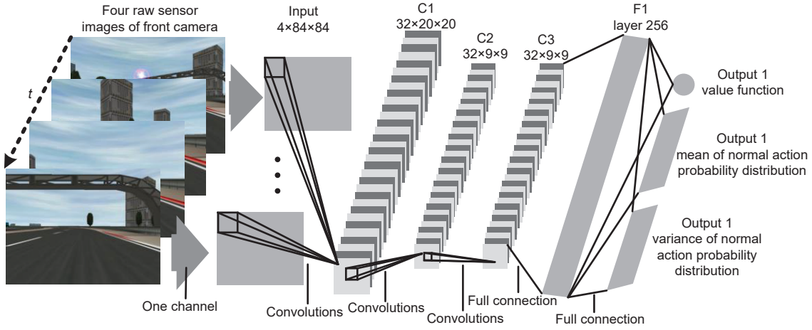
Fig. 2 Architecture of the end-to-end autonomous driving model
